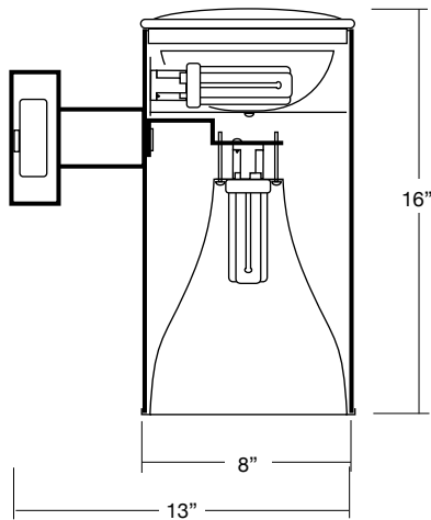
Wall Mount Cylinder (shown w/ WL -Wet Location Lens)
