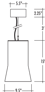
6212D ◆ Fluorescent, Dimming
