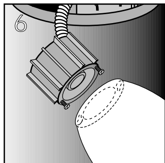
6 Attach reflector to lamp holder by slide into keyhole slots and tighten screws
