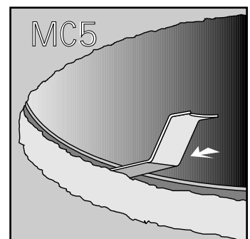
MC5 For frames with no collar, clip slides between frame and ceiling
