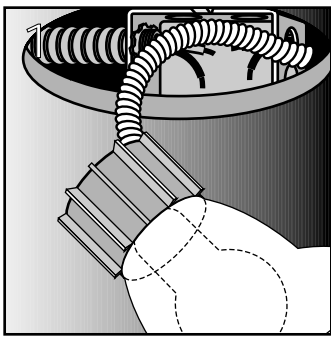
Remove existing reflector (ellipsoidal must be pushed up into ceiling)
