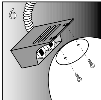
Attach reflector to lamp holder by keyhole slots and tighten screws
