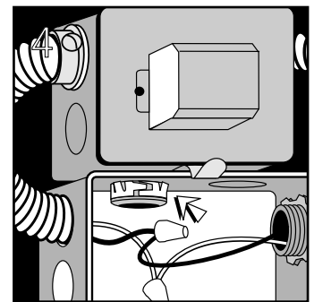
Connect ballast assembly to J-box for support, use box connector
