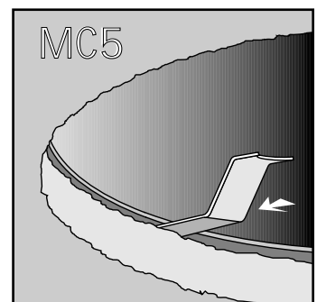
For frames with no collar, clip slides between frame and ceiling
