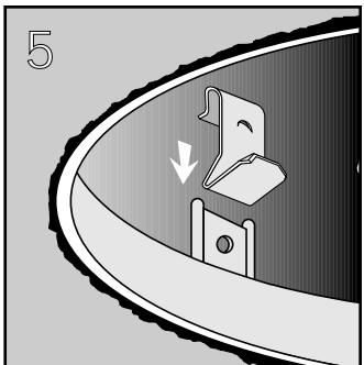
Snap on MC2 spring clips to mounting frame
