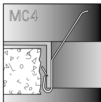
MC4 Clip mounts under mounting frame collar
